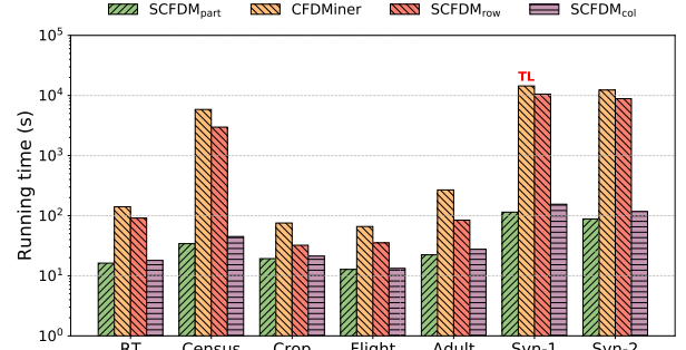
(a) Running time comparison of SCFDM part and baselines
