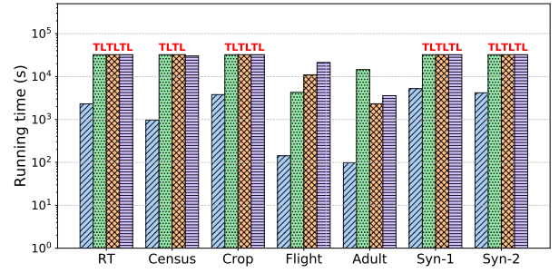
(b) Running time comparison of SCFDM all and baselines
